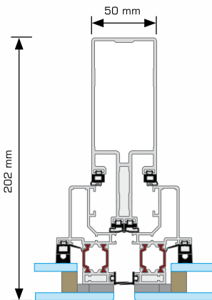
Mullion cross-section
