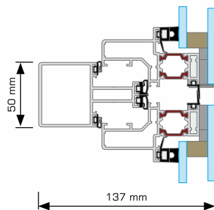
Transom cross-section
